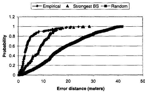
Figure 3 CDF of the error in location estimation.
